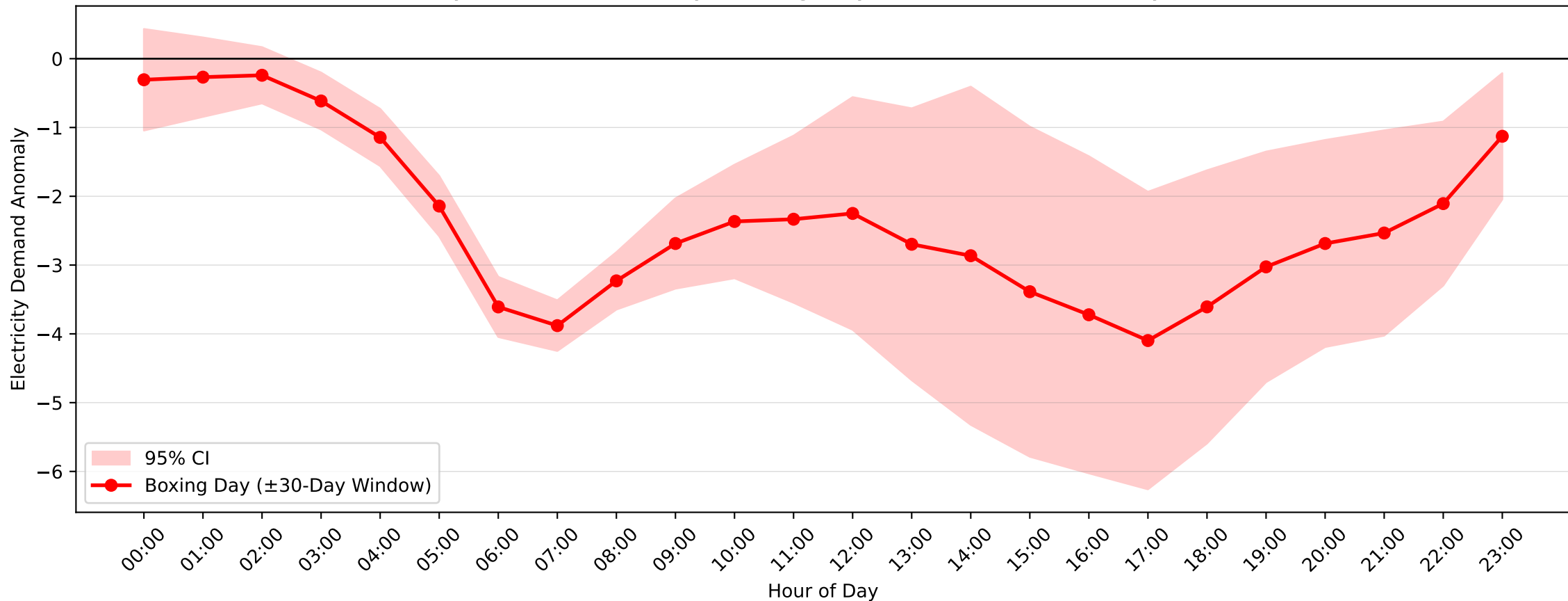
Revesby Demand Anomaly: Boxing Day (2004–2017, \pm 30 -Day Window)
